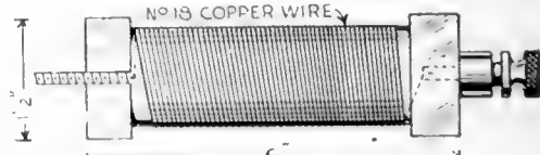
Choke coil consisting of a single layer of about 50 turns of wire wound on a spindle of hard rubber
